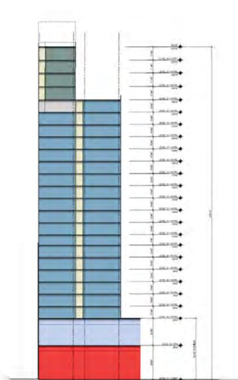
CROSS SECTION 1/16" = 1'-0"
